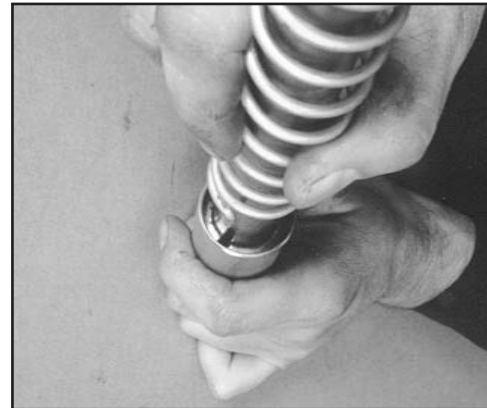
FIG. 48: INSTALL SPRING
